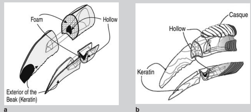
Figure 11. A schematic of the (a) toucan and (b) hornbill beaks.
