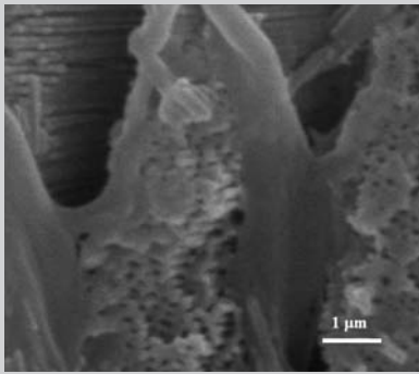
Figure 16. An SEM micrograph of fracture surface showing the twisted plywood (Bouligand) structure of crab exoskeleton.
