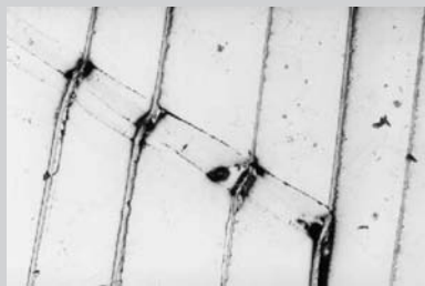
Figure 7. The mechanisms of damage accumulation in nacreous region of abalone. (a, b) Pullout of tiles; (c) plastic microbuckling.
