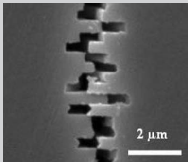
Figure 7. The mechanisms of damage accumulation in nacreous region of abalone. (a, b) Pullout of tiles; (c) plastic microbuckling.
