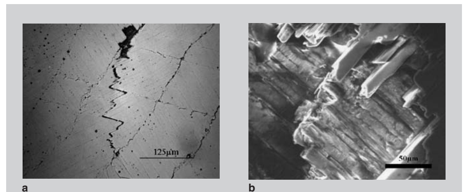
Figure 10. Fracture patterns in a conch shell; (a) crack delocalization shown in polished section and (b) scanning-electron micrograph of fracture surface showing cross lamellar structure.
